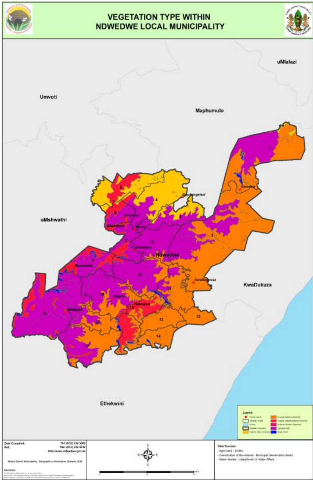
Map 4: Types of Vegetation in Local Municipality
