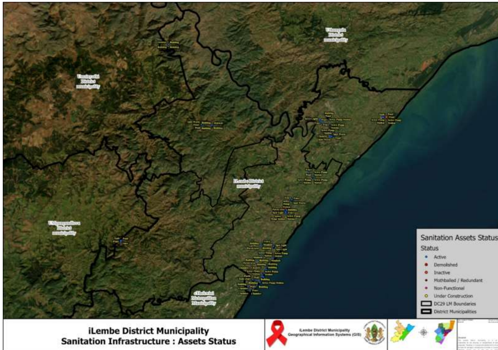
Map 19: Sanitation Water Infrastructure Assets Status
