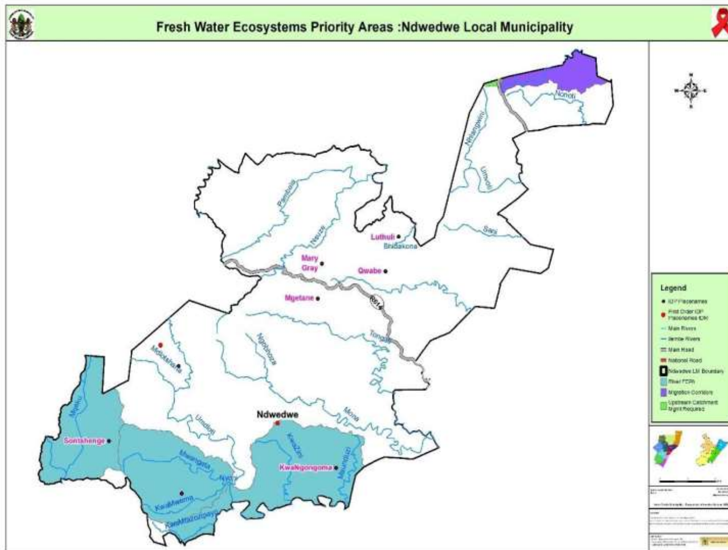
Map 9: Rivers Adapted from EMF: iLembe District Municipality, 2014
